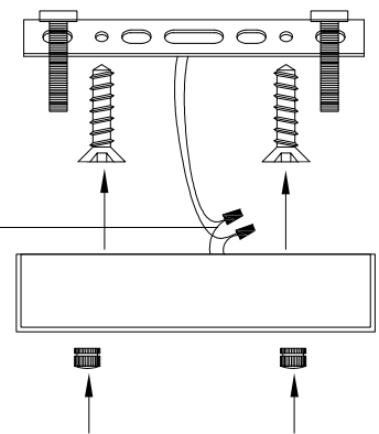
Enlarged Detail
