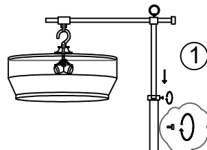
Insert lamp body 1 into lamp body 2 and lock with hand nut
