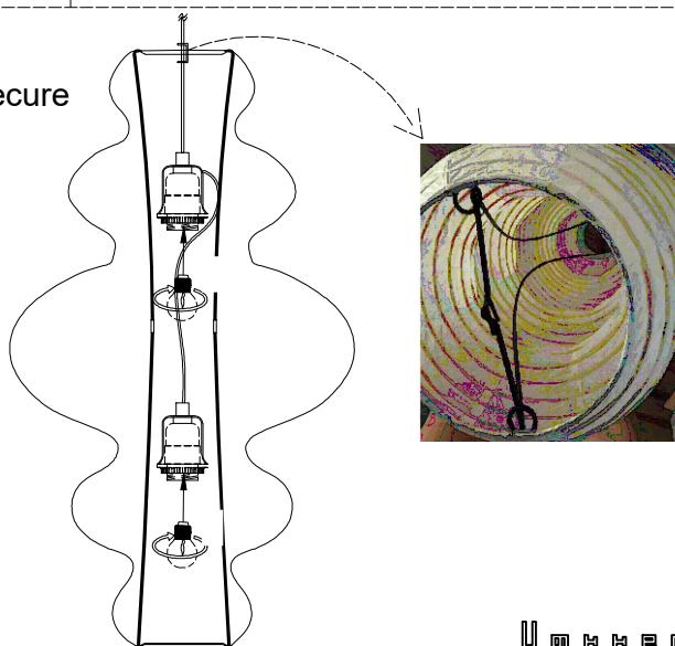
4: Installing bulb
