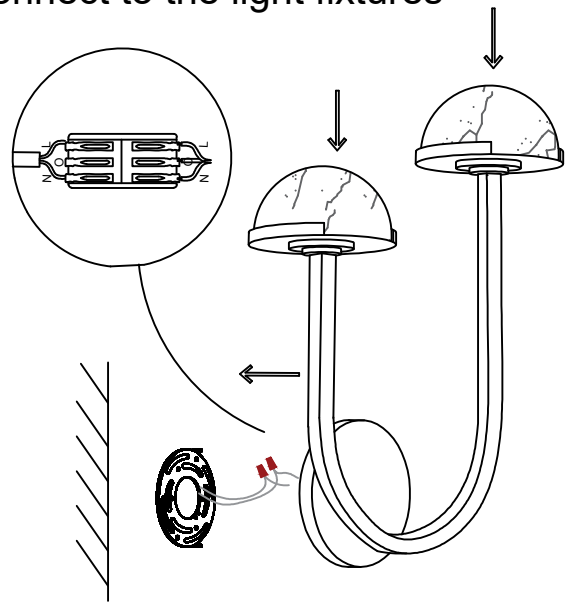
Install the lamp body on the hanging plate
