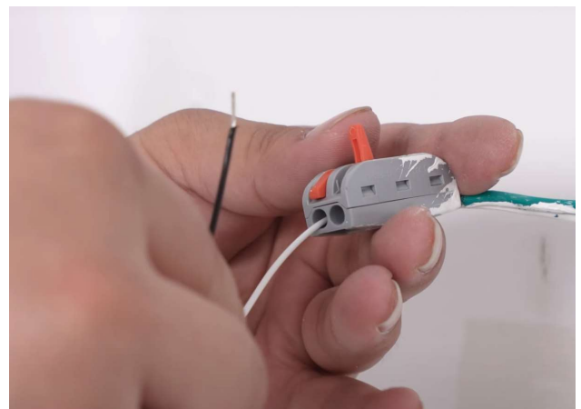
3. Connect the lamp wires to the reserved wires
